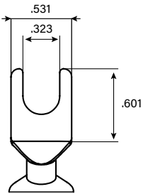
U-Spade Dimensions (in.)
