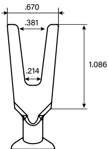
V-Spade Dimensions (in.)
