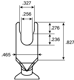
Multi-Spade Dimensions (in.)
